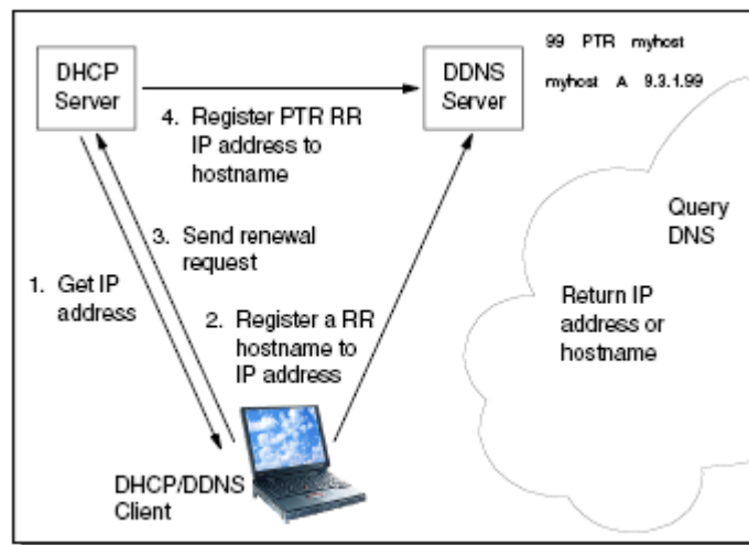
Gambar 9.4 DDNS
