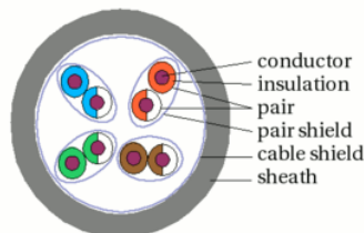
Gambar 3.25 S/STP
