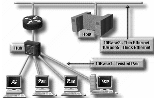
Gambar 3.6 Ethernet IEEE 802.3
