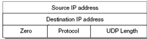
Gambar 7.3 Pseudo IP Header – UDP
