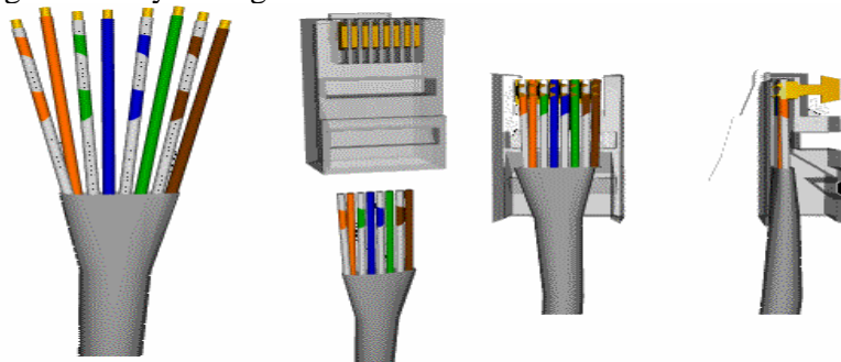
Gambar 3.27 TIA/EIA-586-B
