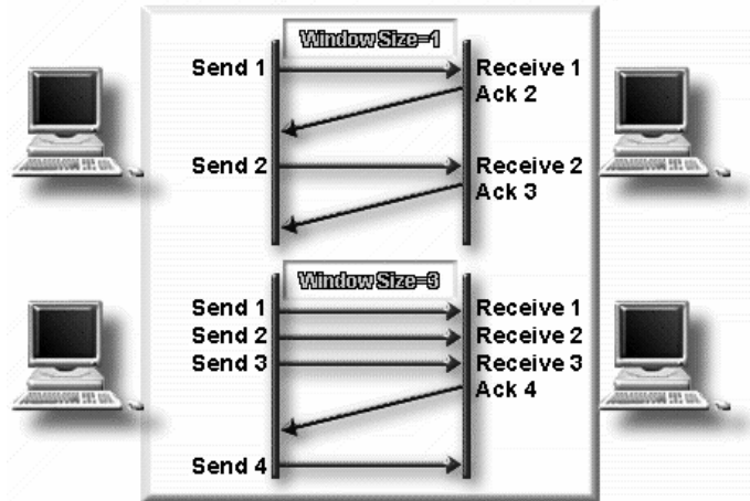
Gambar 2.9 Sistem windowing
