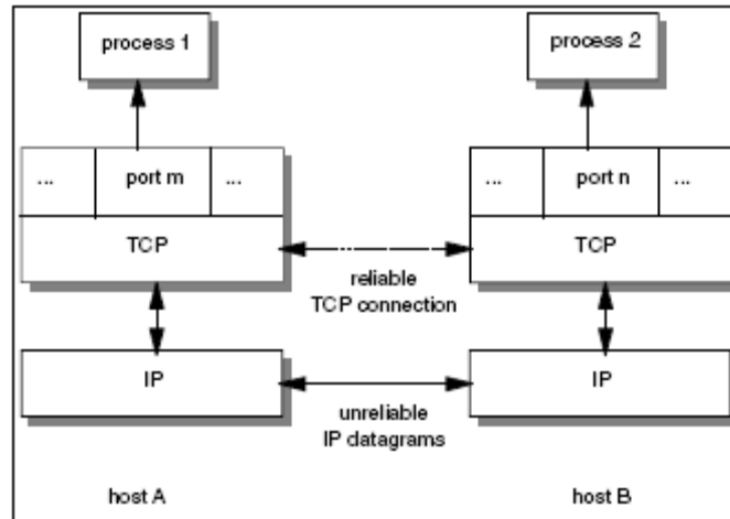
Gambar 7.4 IPC
