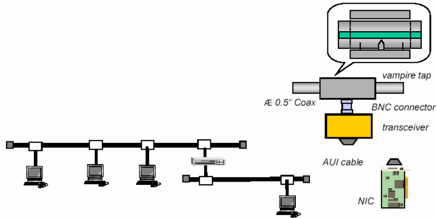
Gambar 3.7 Ethernet 10Base5
