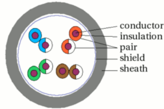
Gambar 3.26 S/UTP
