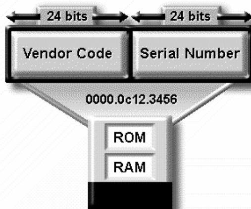
Gambar 2.15 Media Access Control (MAC)
