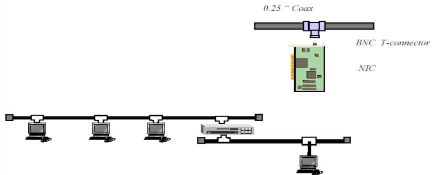
Gambar 3.8 Ethernet 10Base2
