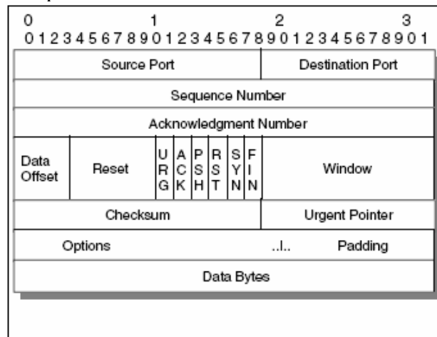
Gambar 7.5 Format TCP
