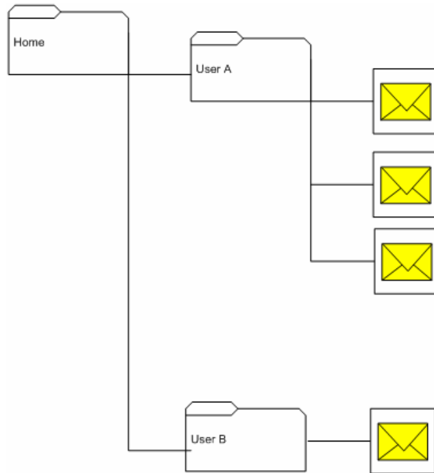
Gambar 12.10 Maildir
