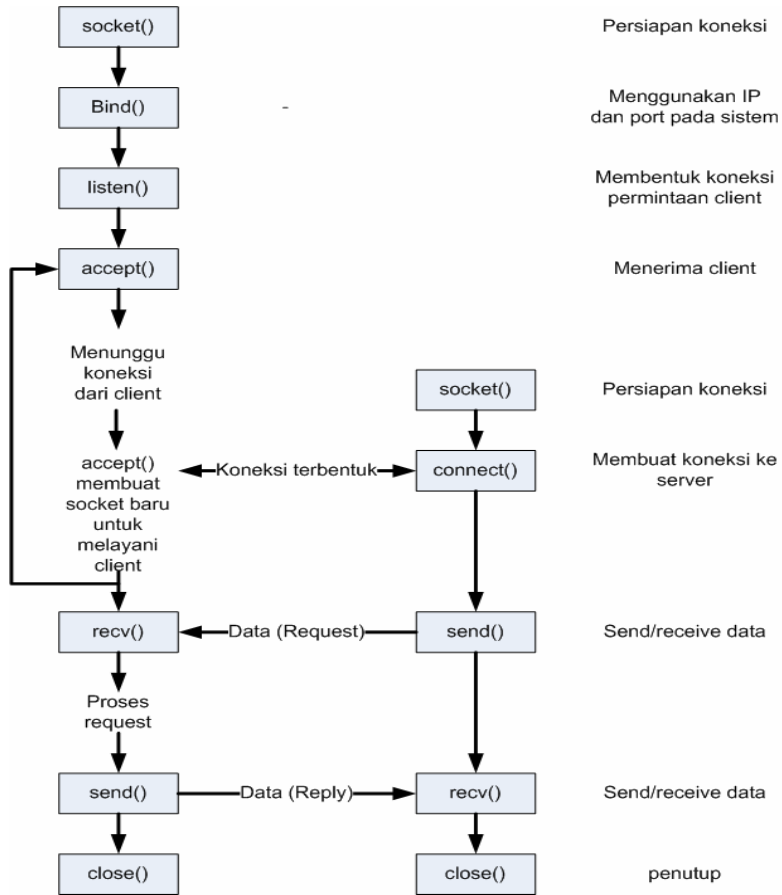
Gambar 8.2 Diagram Alir Program Berbasis Connection-oriented
